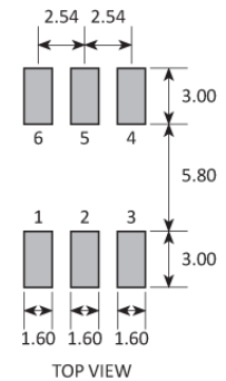
SOLDER PAD LAYOUT
