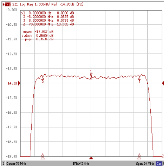
Ripple Variation Fo \pm 8.2MHz
