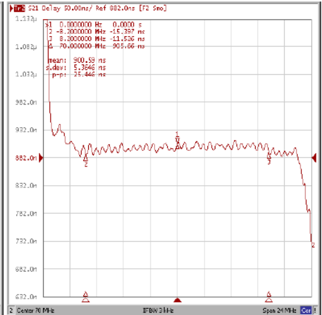
Group Delay Variation Fo \pm 8.2MHz
