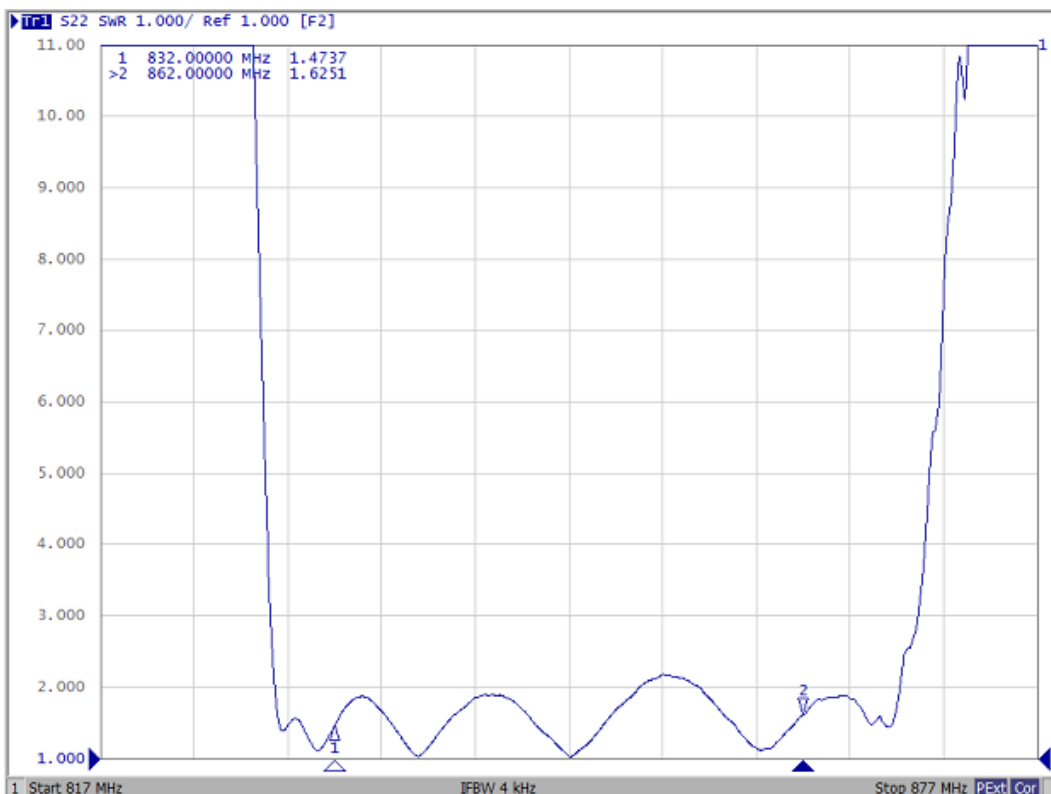
S22 VSWR
