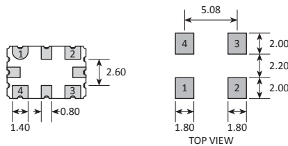
SOLDER PAD LAYOUT
