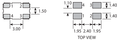
SOLDER PAD LAYOUT
